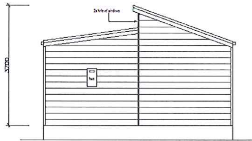
REAR ELEVATION
