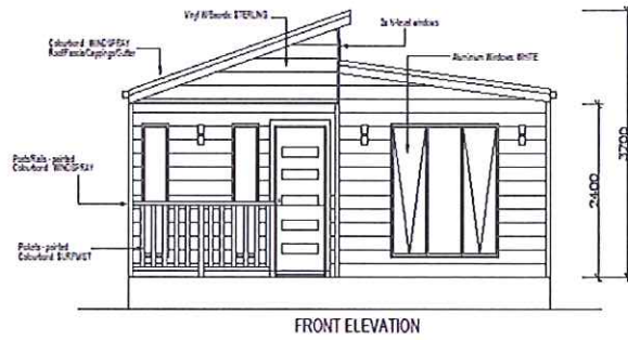
FRONT ELEVATION
